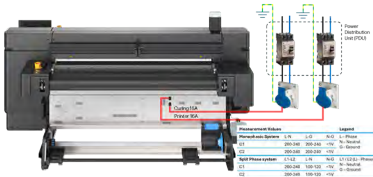
Figure 2-1 Electrical configuration diagram (for reference only)
